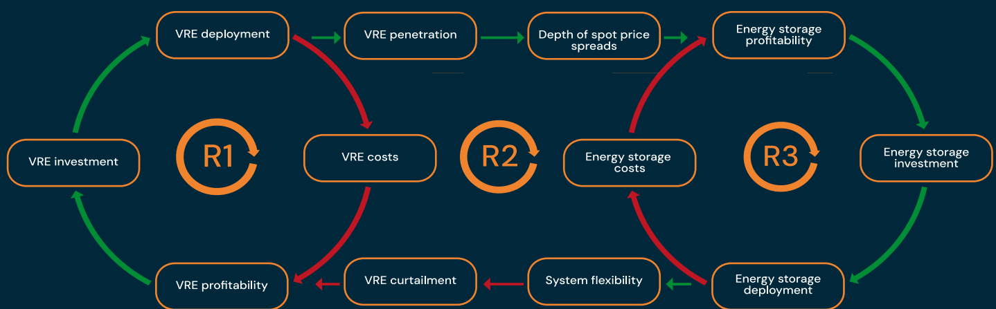
Figure 9: CLD showing the synergistic dynamic between variable renewable energy (VRE) and energy storage deployment. Each technology is subject to its own learning-by-doing reinforcing loop (R1 and R3), but the complementarity between the technologies links these loops to create a larger reinforcing loop (R2). Green arrows represent positive causal relationships (variables move in the same direction) and red arrows represent negative causal relationships (variables move in opposite directions).
