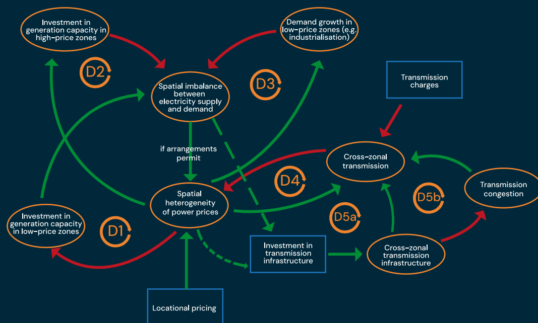
Figure 12: CLD showing multiple dampening feedback loops that act to limit the differences in electricity prices across a certain geographical area. Green arrows represent positive causal relationships (variables move in the same direction) and red arrows represent negative causal relationships (variables move in opposite directions). Dashed lines indicate weak/conditional relationships. Orange nodes represent variables within the system, blue rectangular nodes represent policy inputs.
