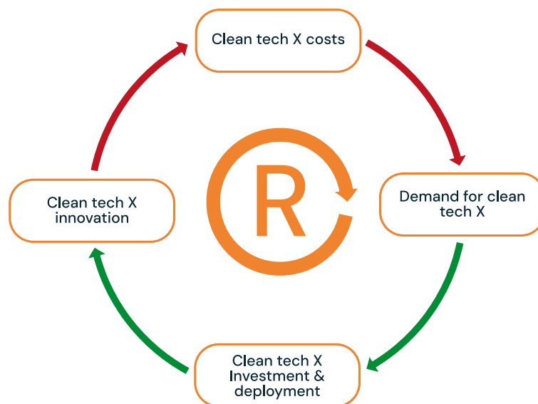
Figure 20: Example of a CLD showing a reinforcing feedback via technology development and diffusion. Green arrows represent positive causal relationships (variables move in the same direction) and red arrows represent negative causal relationships (variables move in opposite directions).
