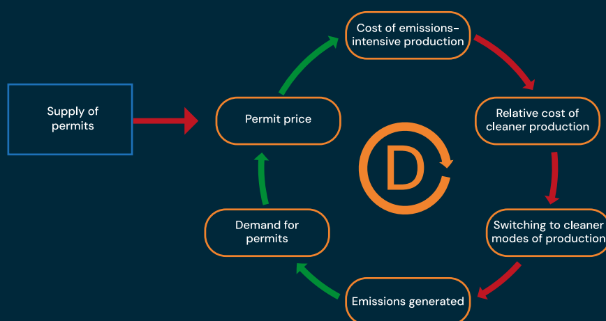
Figure 14: Dampening feedback loop representing the waterbed effect in emissions trading schemes. Green arrows represent positive causal relationships (variables move in the same direction) and red arrows represent negative causal relationships (variables move in opposite directions). Orange nodes represent variables within the system, blue rectangular nodes represent policy inputs.
