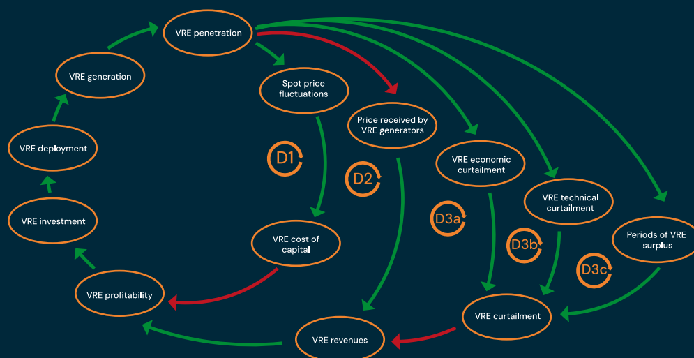
Figure 7: CLD showing the multiple channels through which VRE (variable renewable energy) cannibalisation can occur. Green arrows represent positive causal relationships (variables move in the same direction) and red arrows represent negative causal relationships (variables move in opposite directions).
