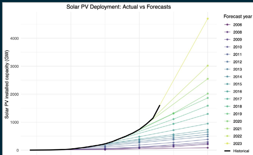
Figure 3: Comparison of global solar power PV deployment projections against actual deployment. Different coloured curves represent projections made in different years. The black, emboldened line shows historical deployment.
