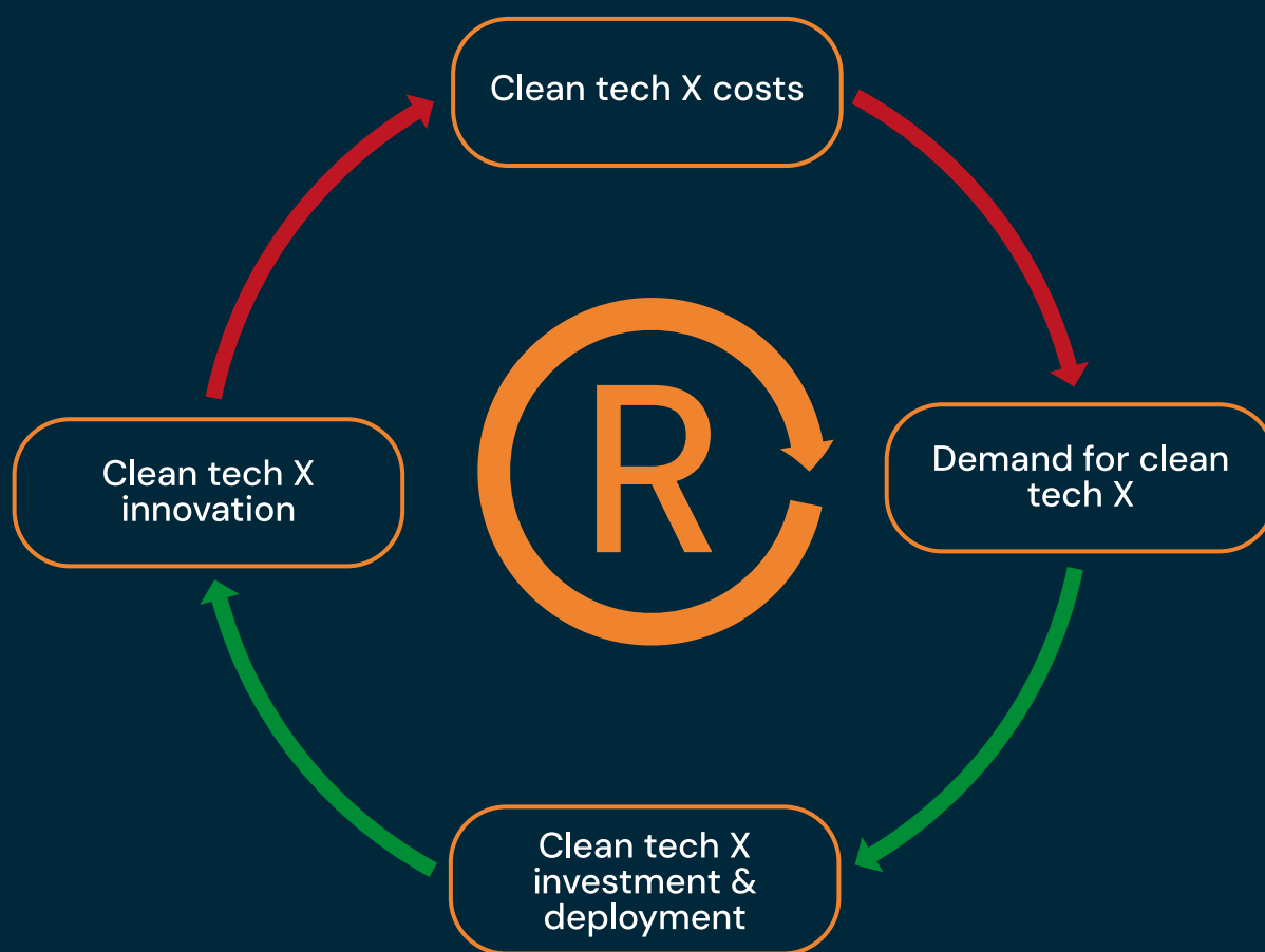
Figure 2: A reinforcing feedback loop of clean technology development and diffusion. Green arrows represent positive causal relationships (variables move in the same direction) and red arrows represent negative causal relationships (variables move in opposite directions).
